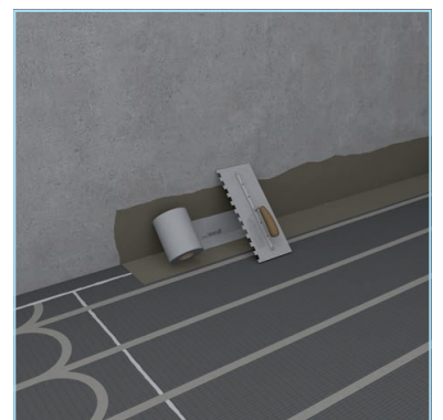
Sealing of wall/floor connections
