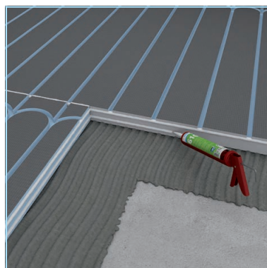
Sealing of joint areas
