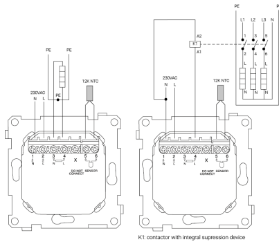
WIRING DIAGRAM
