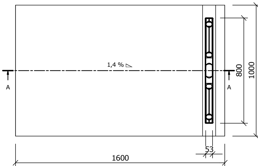
top view ( 1 : 15 )
